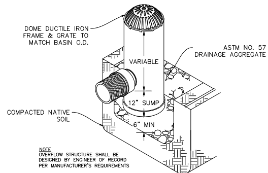
OVERFLOW STRUCTURE
