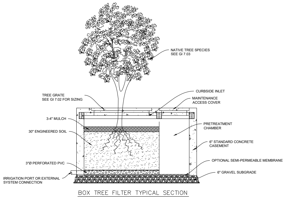
BOX TREE FILTER TYPICAL SECTION
