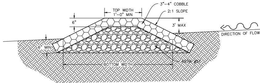
BERM LEVEL SPREADER SECTION
